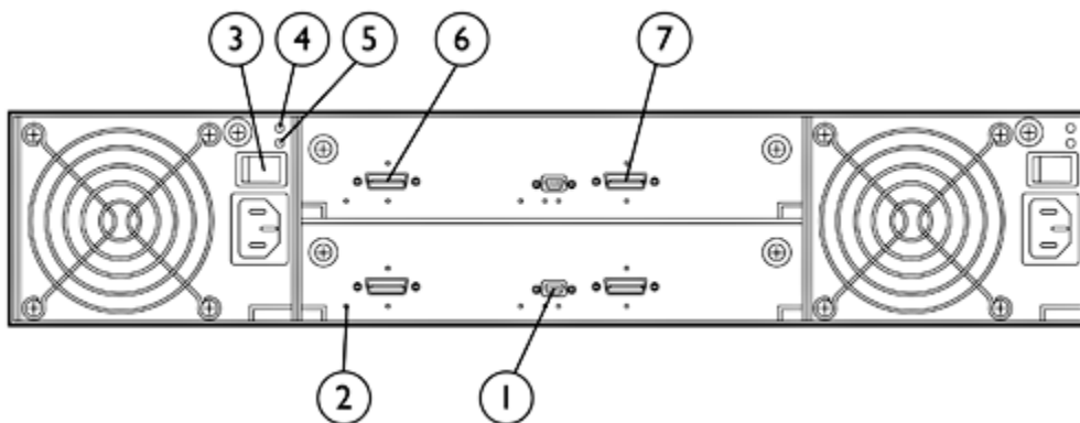
MSA2000 Dual I/O 3.5" 12 Drive Enclosure
